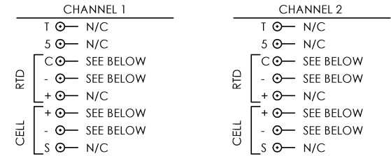
THORNTON TYPE 208 CELL WIRE CONNECTIONS (TYPICAL FOR CHANNELS 1 AND 2)
