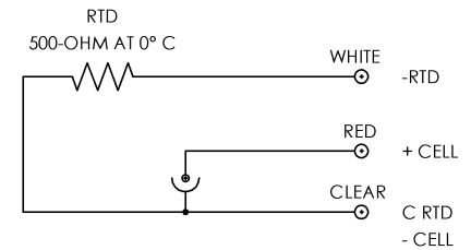
THORNTON TYPE 208 CELL WIRE CONNECTIONS (TYPICAL FOR CHANNELS 1 AND 2)
