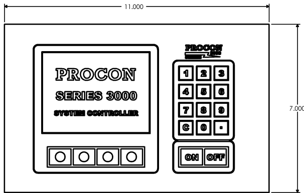
FRONT PANEL
